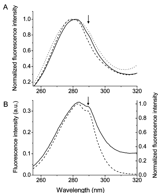
FIGURE 9: Evidence for RET between Trp105 and bound ANS in the L105W-ANS complex. (A) Key: dotted line, corrected excitation spectrum (emission at 500 nm) of ANS (1.5 \mu M) in ethanol; dashed line, corrected excitation spectrum (emission at 500 nm) of the W17Y (5.0 \mu M)-ANS (2.5 \mu M) complex; solid line, corrected excitation spectrum (emission at 500 nm) of the L105W (4.4 \mu M)-ANS (2.5 \mu M) complex. (B) Key: dashed line, excitation spectrum (emission at 348 nm) of L105W (4.4 \mu M) without ANS; solid line, difference excitation spectrum at an emission of 500 nm [spectrum of L105W-ANS - 0.67(spectrum of the W17Y-ANS complex shown in (A))]. The arrow indicates the position of the 0-0 band of the ^1L_b electronic absorption transition of Trp.
