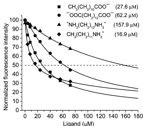
FIGURE 13: Displacement of DAUDA from the DAUDA(2 \mu M)–TL(4 \mu M) complex by various ligands at pH 7.3. Excitation and emission wavelengths were 345 and 498 nm, respectively. IC_{50} values for each ligand are shown in parentheses. Solid curves are generated by fitting of the experimental data to one binding site model.
