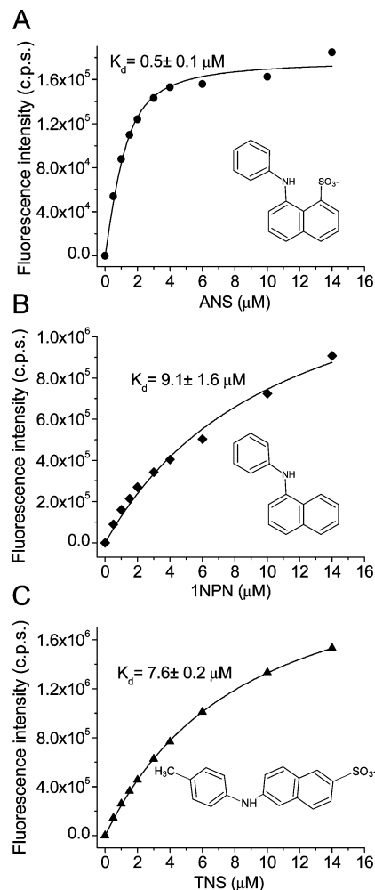
FIGURE 4: Binding curves of the fluorescence probes ANS (A), 1NPN (B), and TNS (C) to apoTL (5 μM). Emission \lambda values for ANS, 1NPN, and TNS binding were 465, 416, and 432 nm, respectively.
