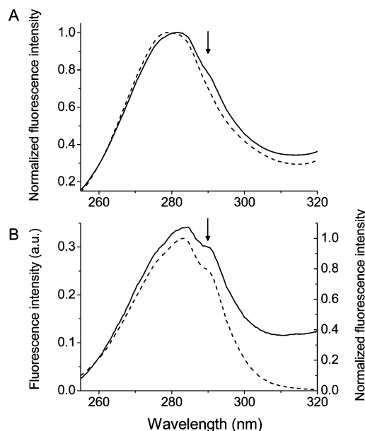
FIGURE 10: Evidence for RET between Trp101 and bound ANS in the C101W-ANS complex. (A) Key: dashed line, corrected excitation spectrum (emission at 500 nm) of the W17Y (5.0 \mu M)-ANS (2.5 \mu M) complex; solid line, corrected excitation spectrum (emission at 500 nm) of the C101W (5.0 \mu M)-ANS (2.5 \mu M) complex. (B) Key: dashed line, excitation spectrum (emission at 337 nm) of C101W (5.0 \mu M) without ANS; solid line, difference excitation spectrum at an emission of 500 nm [spectrum of C101W-ANS - 0.63(spectrum of the W17Y-ANS complex shown in (A))].
